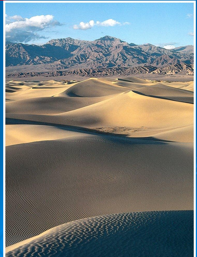
Figure 5-9 Earth System History, Second Edition © 2005 W.H. Freeman and Company
